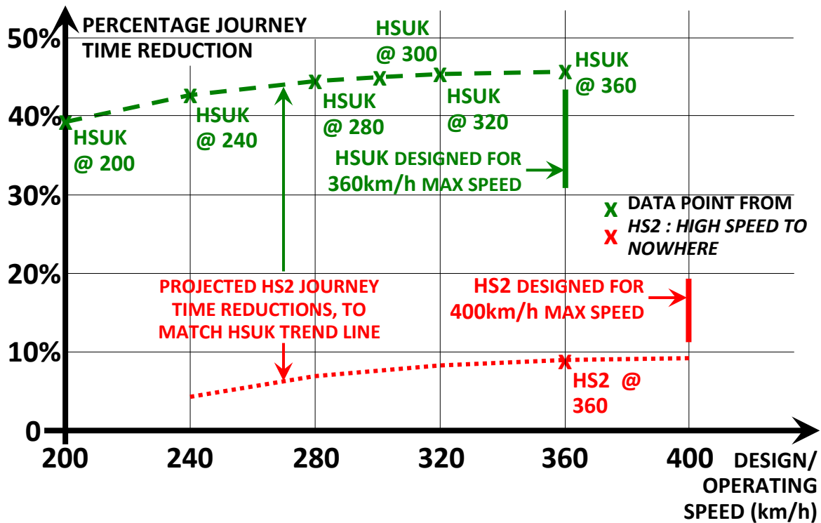
Figure 1 : Relationship between Average Journey Time Reduction and Operating Speed (data from Figure 5.66, P141, HS2 : High Speed to Nowhere)
